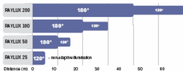
ILLUMINATION DISTANCES
