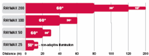
ILLUMINATION DISTANCES
